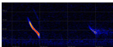
Figure 5: Examples of spectrograms of the recorded species. A spectrogram shows the frequency contour of a signals (call) in time. Most bat species in NW Europe can be identified by their call characteristics.
